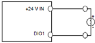
Sinking output
