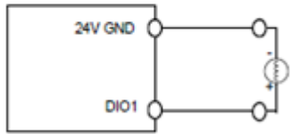
Sourcing output
