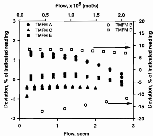
FIG. 3. Deviations of the manufacturers' nitrogen calibrations of IMFM's from the NIST measured values. TMFM's A, C, and E data correspond to the left axis and TMFM's B and D data correspond to the right axis.
