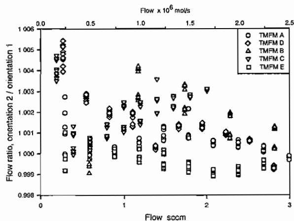
FIG 4 Flow ratio of the TMFM's when calibrated in orientation 2, sensing tube perpendicular to gravity from their calibration in orientation 1, sensing tube parallel to gravity with the flow coincident with gravity
