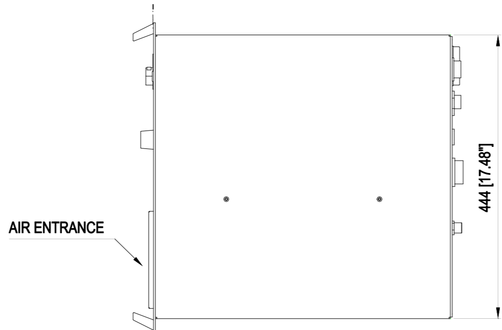
Dimensional Drawing — Note: Unless otherwise specified, dimensions are nominal values in millimeters (inches referenced).
