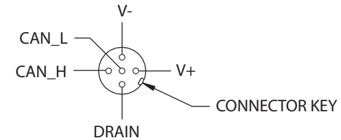
PinOut For DeviceNet™
