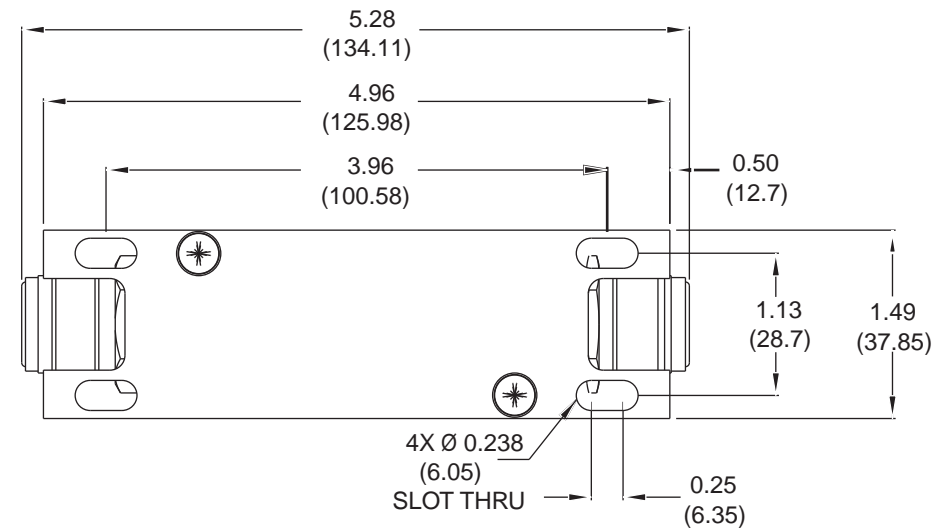
BOTTOM VIEW WITH 8 VCR FITTINGS 4 PLACES (INCLUDES 0.12 THK. MOUNTING PLATE AND (2) SCREWS)
