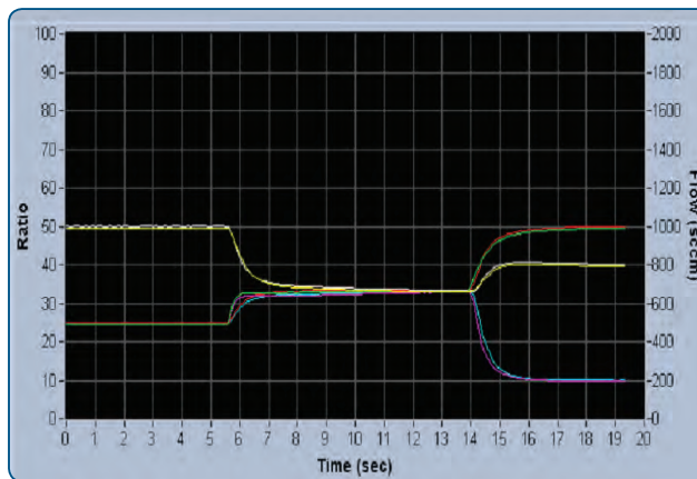
Figure 2 — The DELTA III ratio controller provides control for three channels of flow. Above the device starts with flows of 25, 25 and 50% in channels Q1, Q2, and Q3, respectively. The flow then transitions to 33.3% in each channel followed by a transition to 10, 50 and 40% in each channel, respectively.
