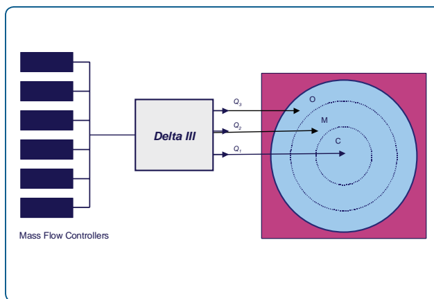
Figure 1 — The above schematic shows how the DELTA III Flow Ratio Controller can be used to control flow to three zones (Center (C), Middle (M) & Outer (O) within a chamber to optimize process uniformity.
