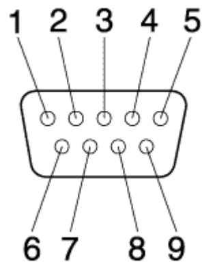
9-pin Accessory Connector
